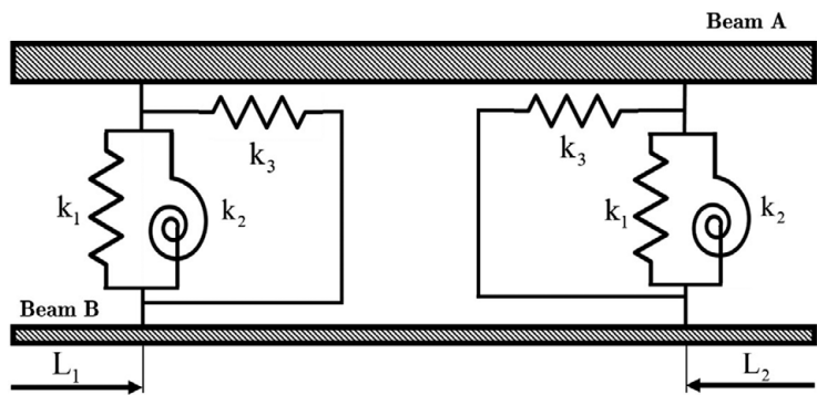
Figure 19. Theoretical model of a coupled beam structure.
